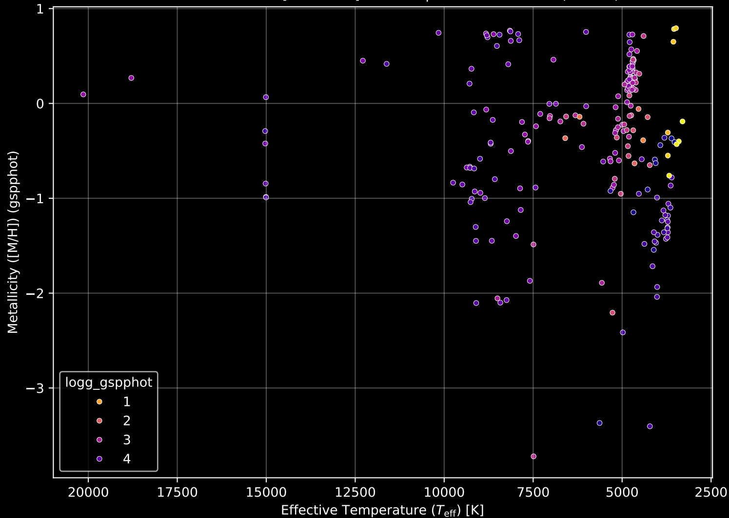
APOGEE DR17 Field: [358+02-O] Stellar Population Parameters (n= 215)
