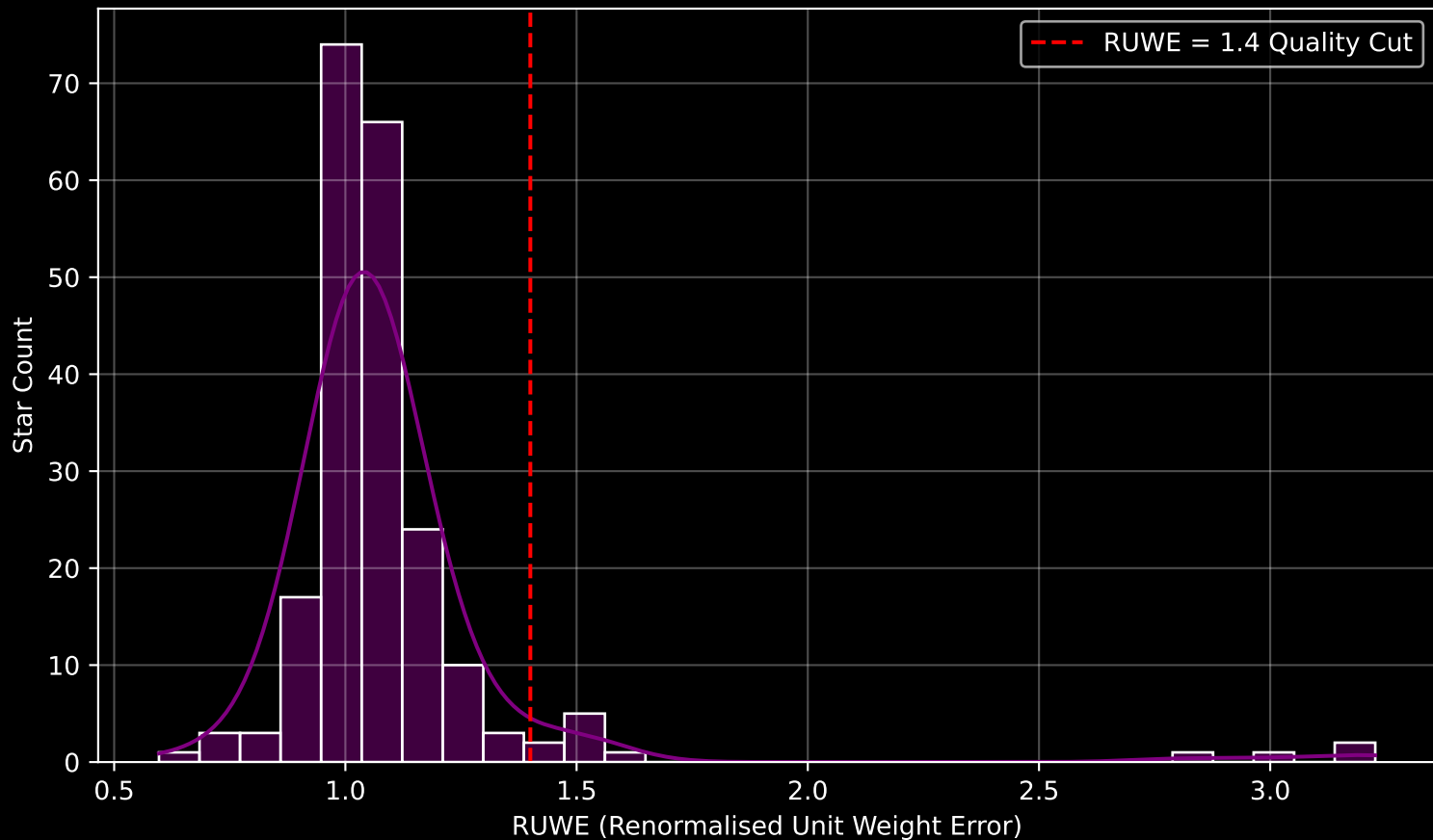
GAPOGEE DR17 Field [358+02-O] RUWE Distribution (n= 213)
