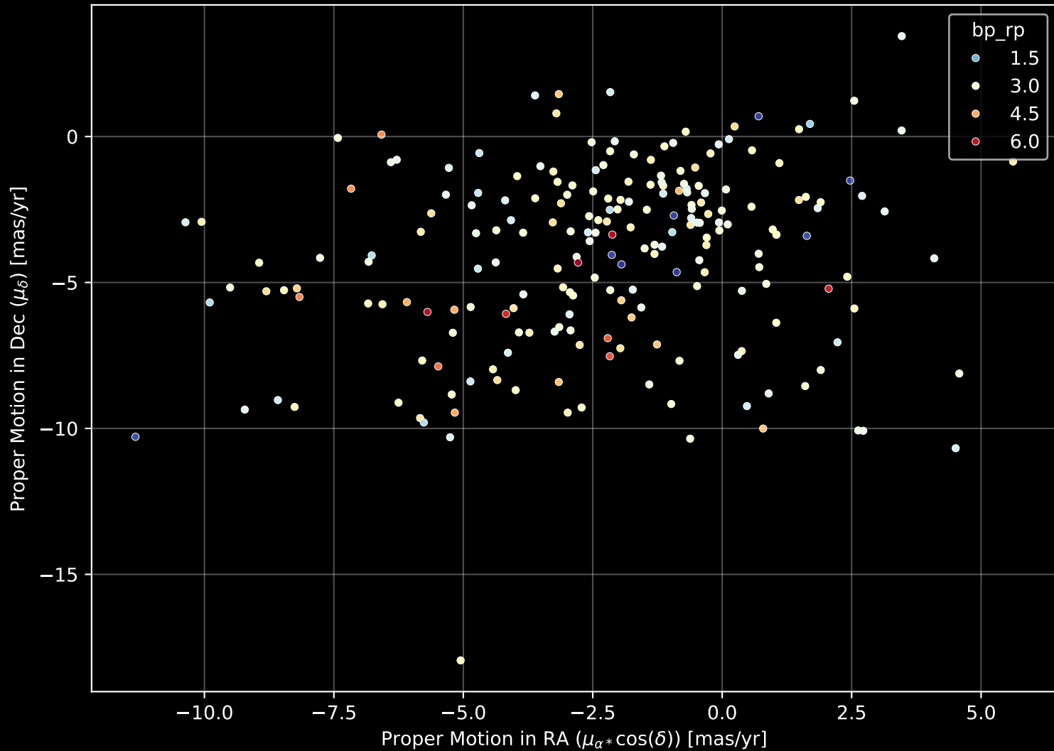
APOGEE DR17 Field: [358+02-O] Proper Motion Diagram (n= 215)
