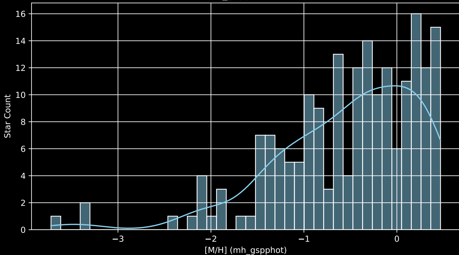
APOGEE DR17 Field: [358+02-O [M/H] (mh_gspphot) (n= 192)
