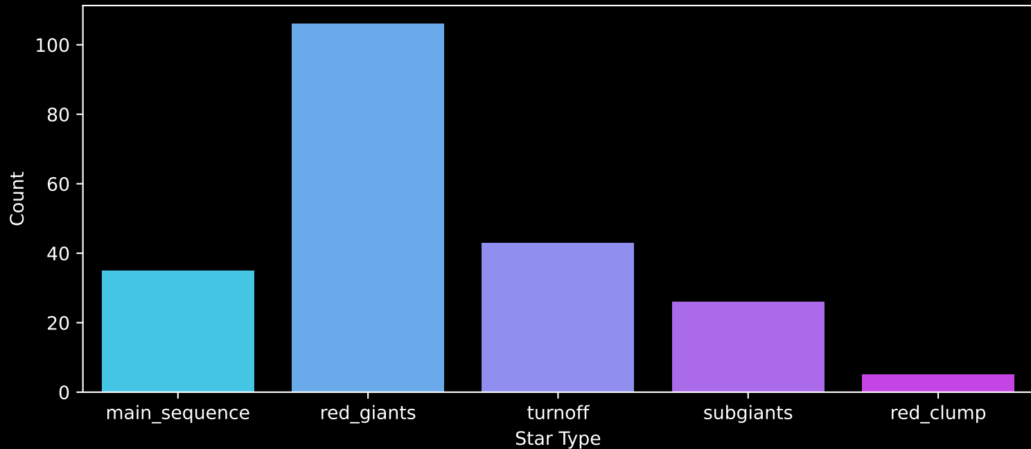
APOGEE DR17 Field: [358+02-O] Count plot of Star Type
