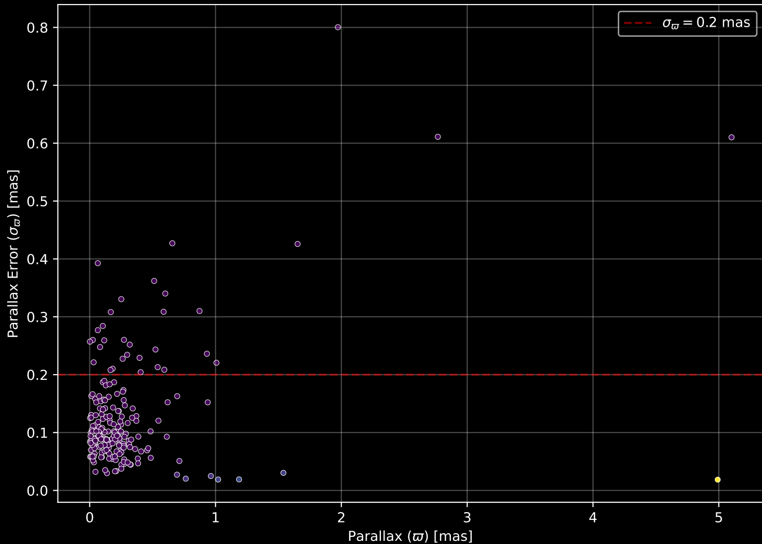
APOGEE DR17 Field: [358+02-O] Parallax Quality (n= 215)
